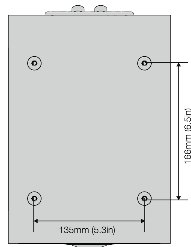
BASE STAND SCREW ALIGNMENT
