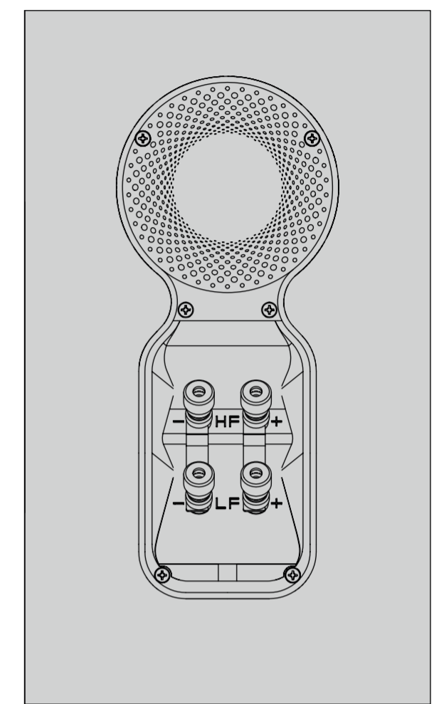
BACK
