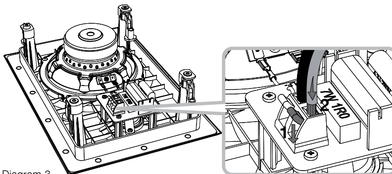
Diagram 3 Cable connection
